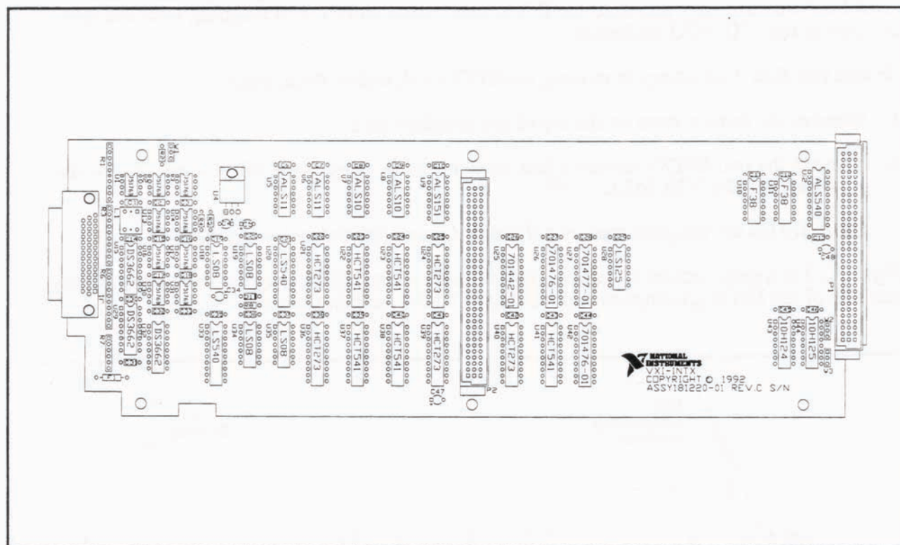
Figure C-3. VXI-MXI INTX Parts Locator Diagram (Front View)
