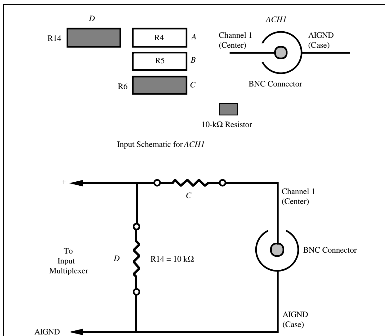
Figure 3-11. Attenuator for Use with BNC-2081 Board Inputs
