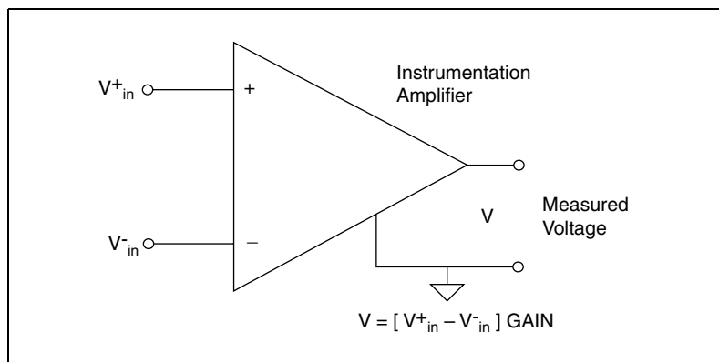
Figure 3-2. DAQCard-700 Instrumentation Amplifier
