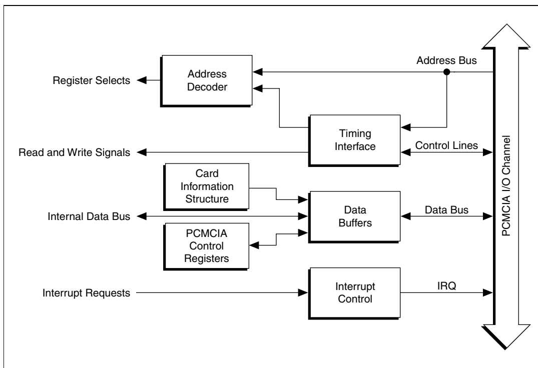
Figure 4-2. PCMCIA I/O Interface Circuitry Block Diagram
