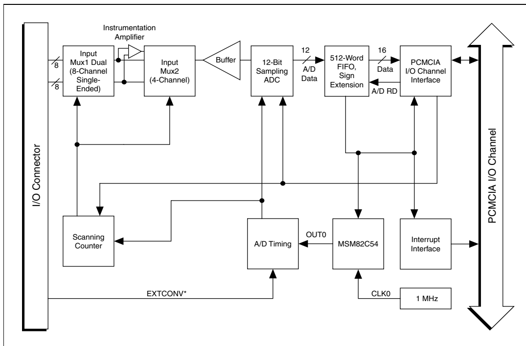
Figure 4-3. Analog Input and DAQ Circuitry Block Diagram
