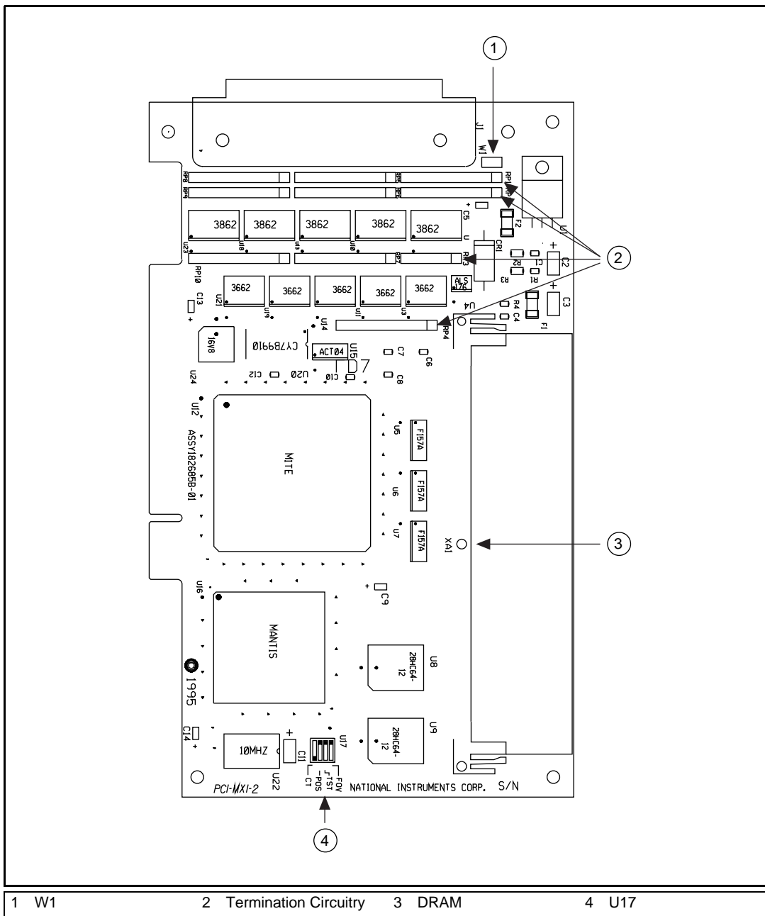
Figure 3-1. PCI-MXI-2 Parts Locator Diagram
