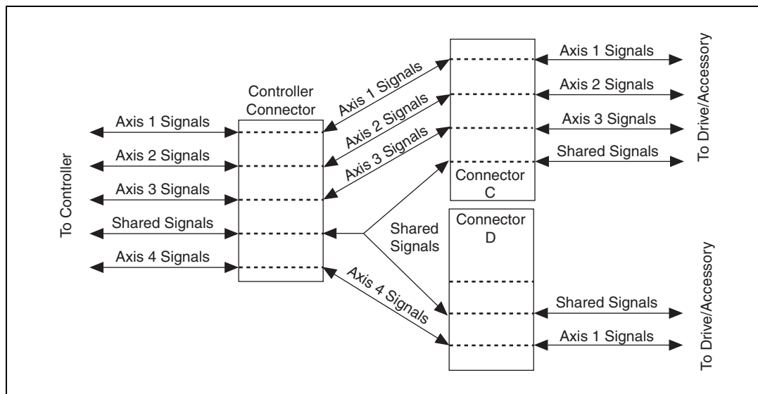
Figure 3. 3 + 1 Connectivity Option
