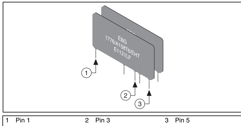
Figure 1. SCXI-1313A Resistor Network Pin Designations
