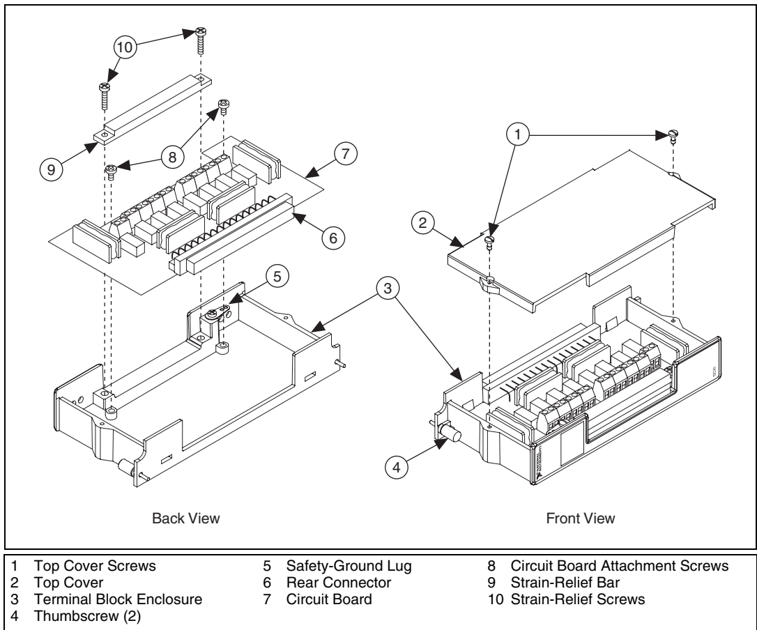
Figure 2. SCXI-1313A Parts Locator Diagram
