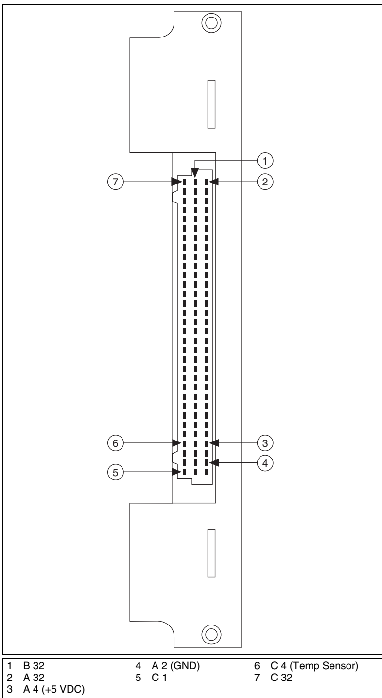
Figure 4. SCXI-1313A Connector Pin Assignments
