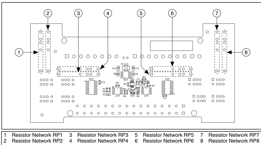
Figure 3. Resistor Network Locator Diagram
