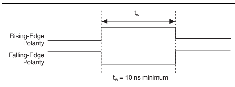
Figure 4-17. TRIG2 Input Signal Timing
