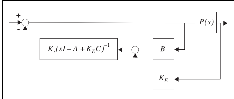
Figure 4-3. C(s) Implemented to Display Left MFD Representation
