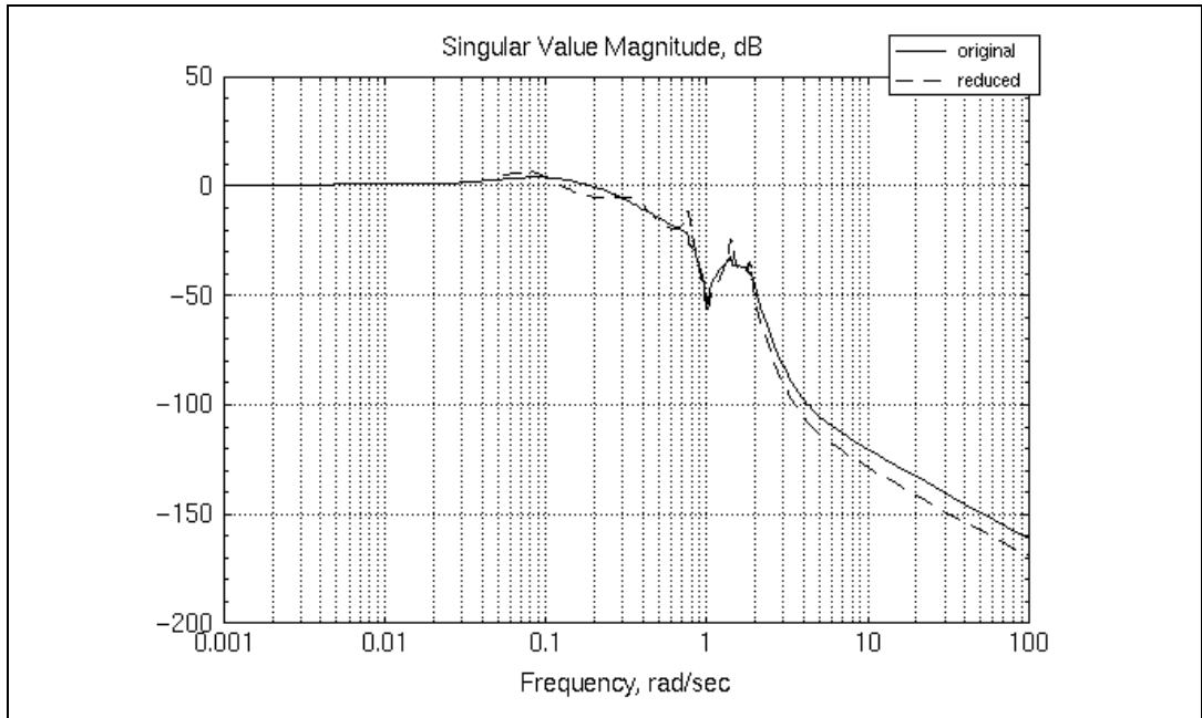
Figure 6-17. Closed-Loop Response with fracted
