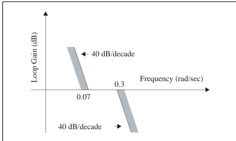
Figure 6-1. Loop Gain Constraints
