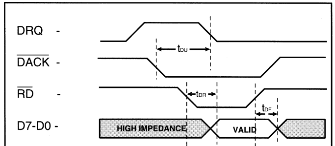
Figure 4. DMA Read
