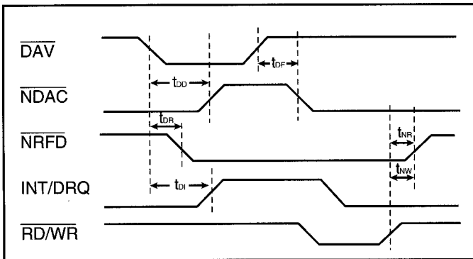
Figure 8. Acceptor Handshake
