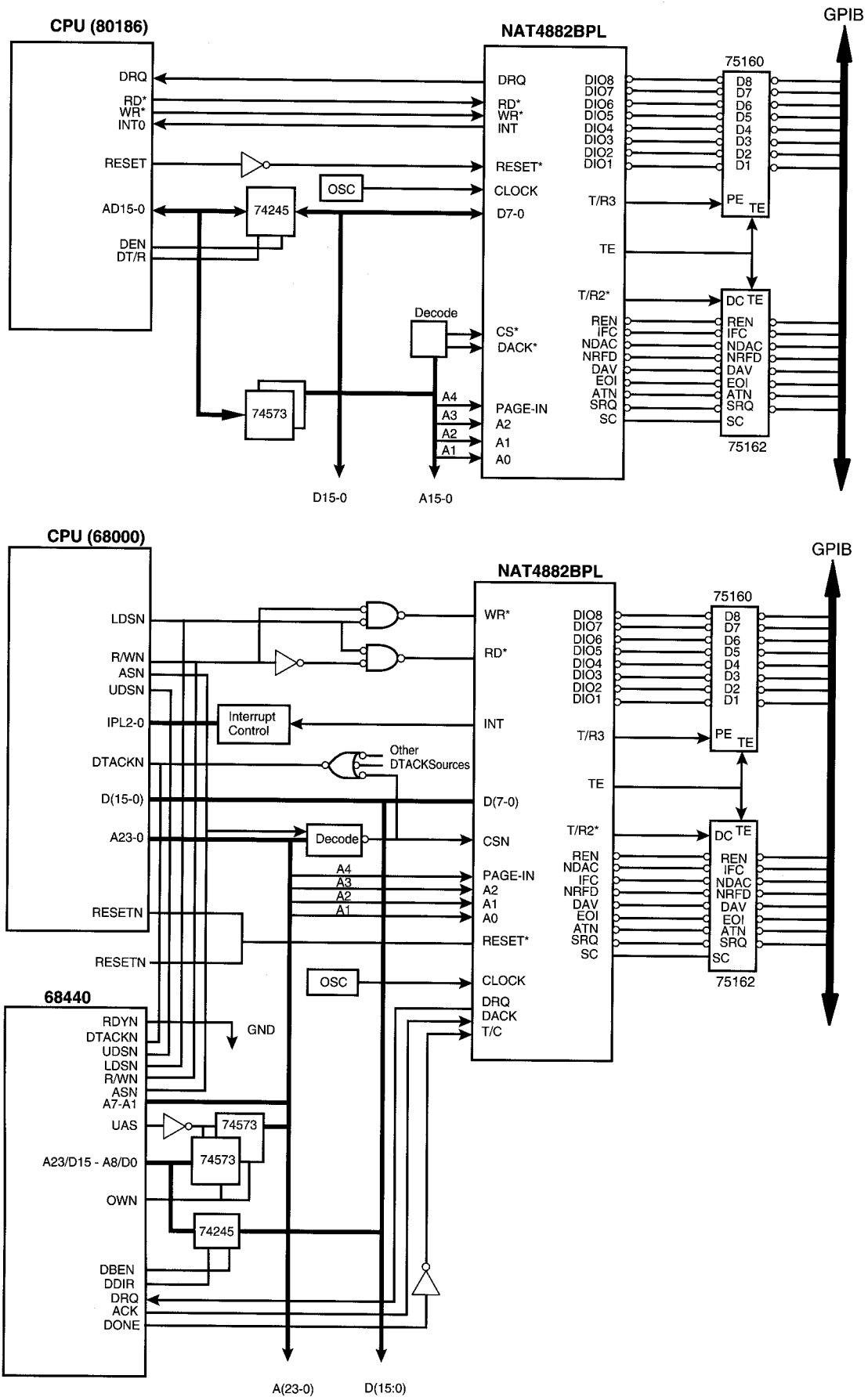
Figure 9. Typical CPU Systems with NAT4882 BPL
