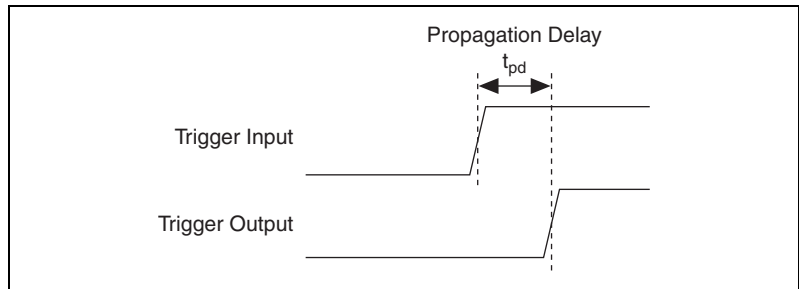
Figure 3-6. Asynchronous Routing Operation
