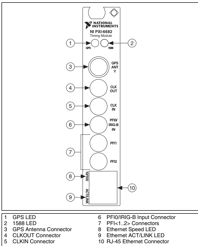
Figure 3-3. NI PXI-6682 Front Panel
