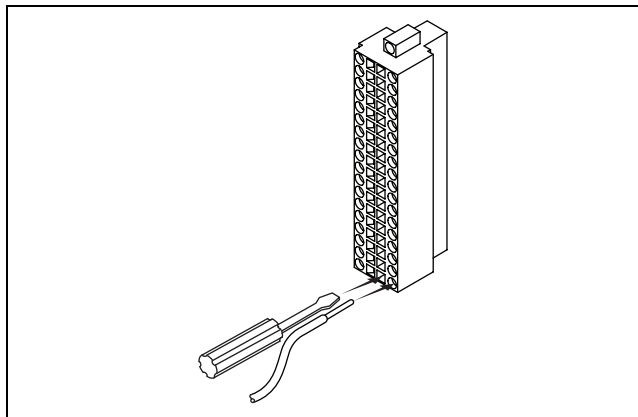
Figure 6. Connecting a Wire to the Spring-Terminal Connector of the cFP-CB-2
