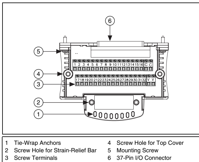
Figure 1. cFP-CB-1 Parts Locator Diagram
