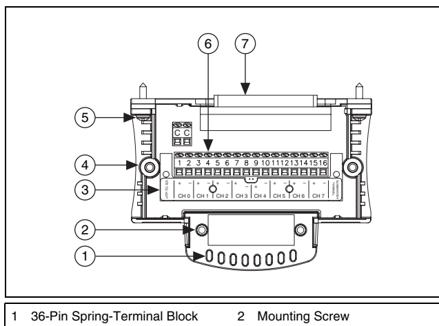
Figure 2. cFP-CB-2 Parts Locator Diagram
