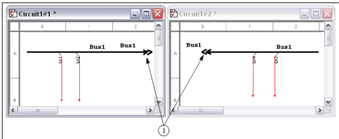
1 Bus Off-Page Connectors
