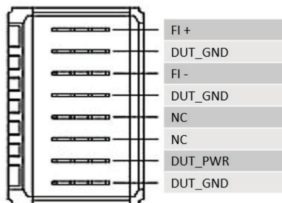
Figure 4, XJ3 Pinout
