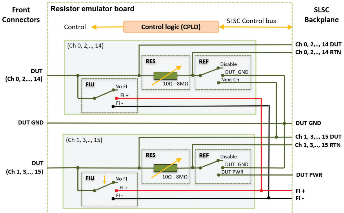
Figure 1, Block diagram
