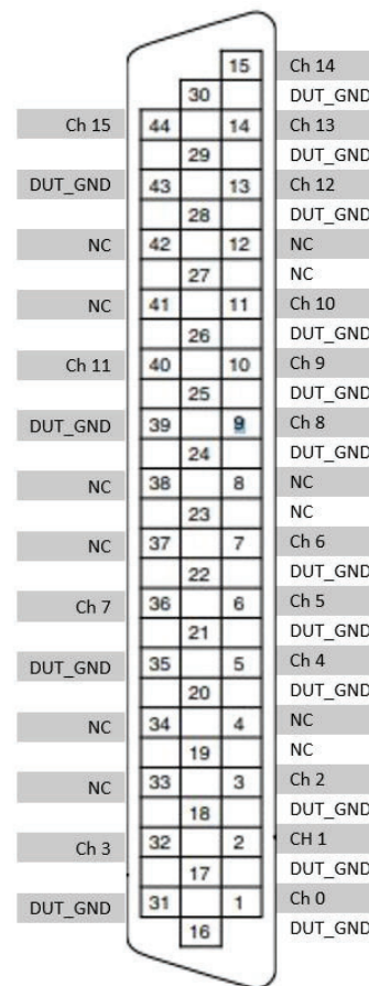
Figure 3, J1 & J2 Pinout
