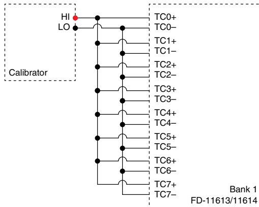
Figure 3. Bank 1 Voltage Channel Adjustment Connections
