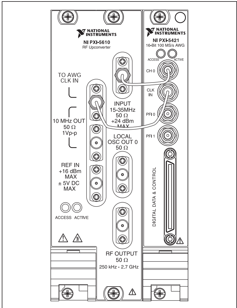
Figure 7. NI PXI-5670/5671 Front Panel
