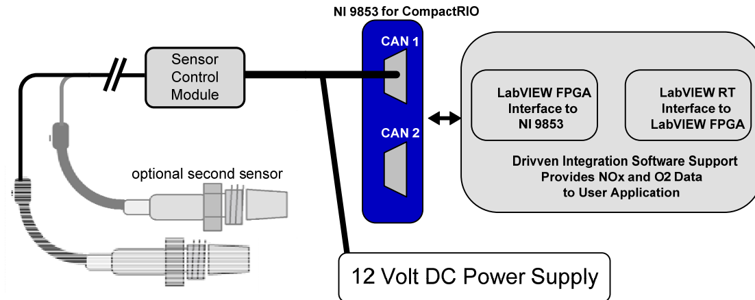
Figure 1 cRIO System Drawing
