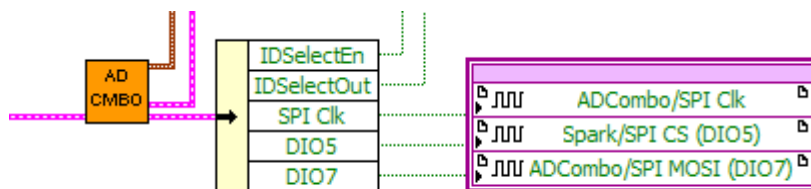
Figure 5. Representative FPGA output node for ADCombo with incorrect output item selection for DIO5. This will cause strange behavior or damage to the spark module. Applying meaningful names to the modules within the project can help identify these coding mistakes.
