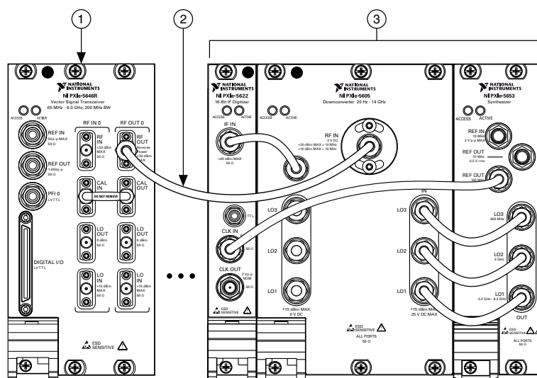
Figure 16 : Output Second Harmonics Verification Cabling Diagram
