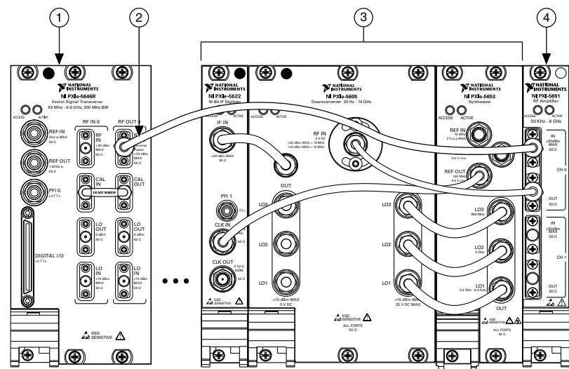
Figure 15 : Output Noise Density Verification Cabling Diagram
