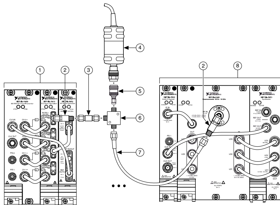
Figure 6 : Connection Diagram for Measuring Splitter Output 1 Power
