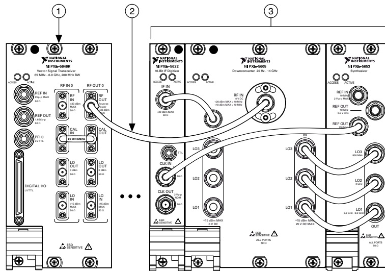
Figure 9 : RF Output Spectral Purity Verification Cabling Diagram
