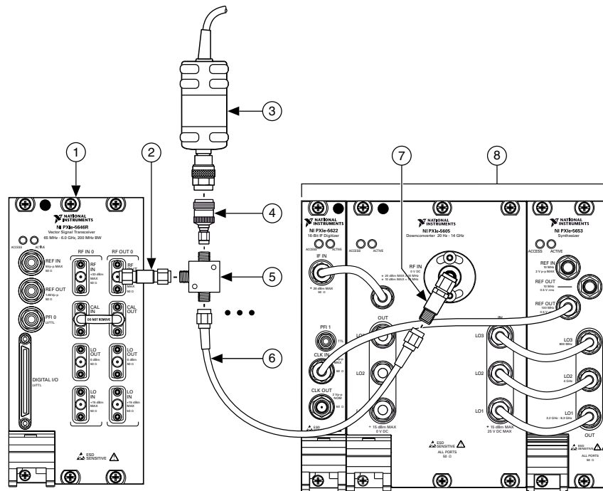
Figure 14 : Output Frequency Response Verification Cabling Diagram
