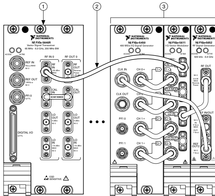
Figure 24 : Internal Frequency Reference Adjustment Cabling Diagram
