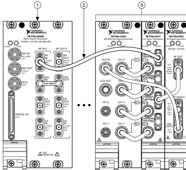
Figure 7 : Internal Frequency Reference Verification Cabling Diagram
