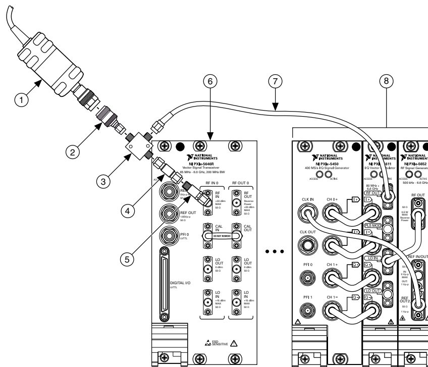
Figure 10 : Input Absolute Amplitude Accuracy Verification Cabling Diagram
