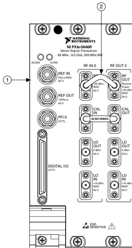
Figure 19 : Residual LO Power and Residual Sideband Image Verification Cabling Diagram
