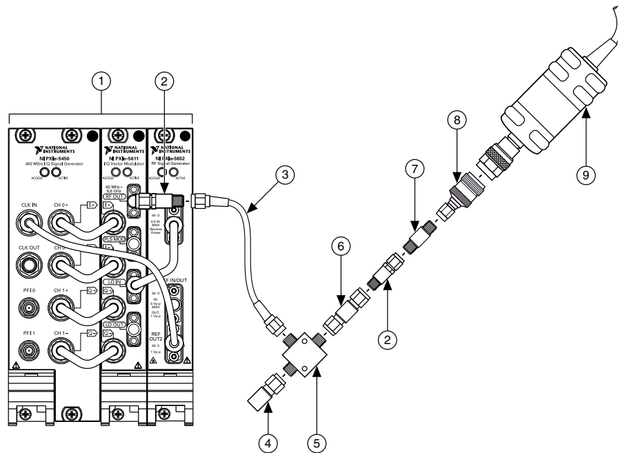
Figure 3 : Connection Diagram for Measuring at Splitter Output 2
