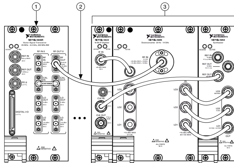
Figure 17 : Output Nonharmonic Spurs Verification Cabling Diagram
