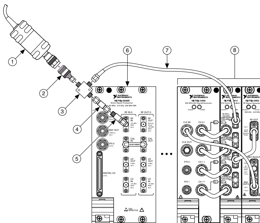
Figure 25 : Absolute Amplitude Accuracy Adjustment Cabling Diagram
