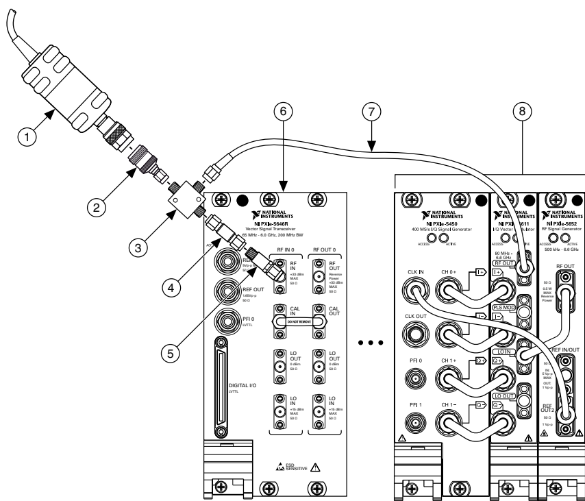
Figure 11 : Input Frequency Response Verification Cabling Diagram
