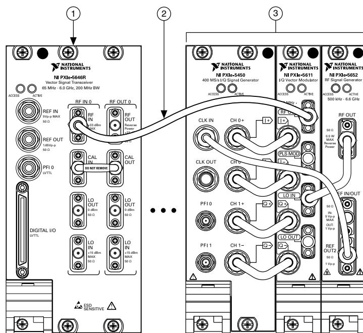
Figure 12 : Input Nonharmonic Spurs Verification Cabling Diagram
