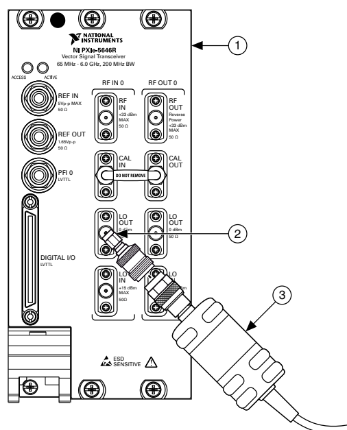
Figure 22 : LO OUT (RF IN 0) Verification Cabling Diagram
