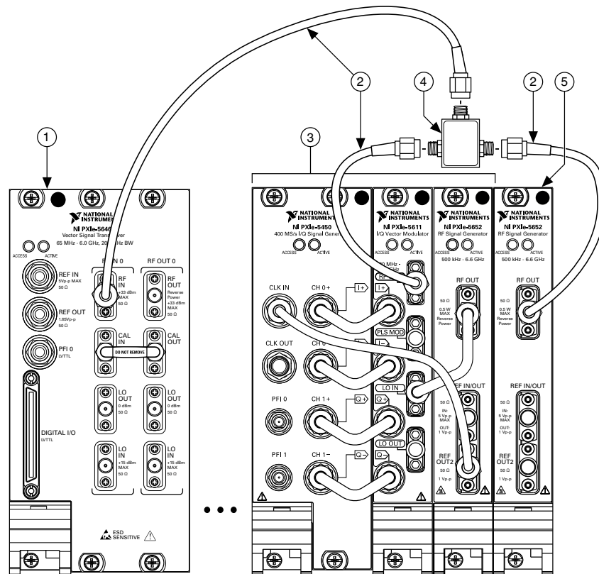
Figure 23 : RF Input IMD3 and IMD2 Verification Cabling Diagram
