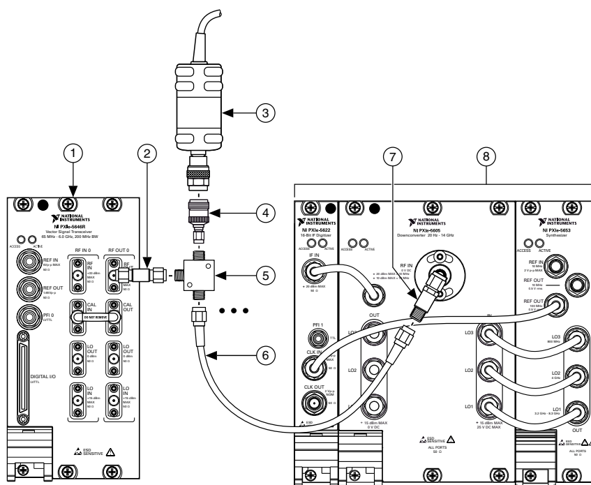
Figure 26 : Output Power Level Accuracy Adjustment Cabling Diagram
