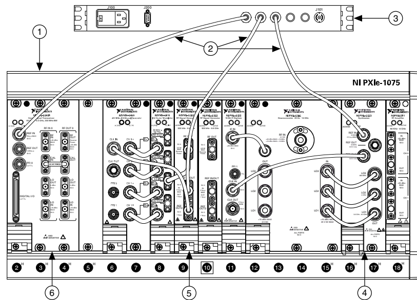
Figure 2 : Connecting Hardware for 10 MHz Reference Connections
