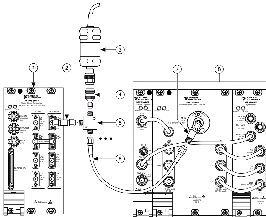
Figure 13 : Output Power Level Accuracy Verification Cabling Diagram
