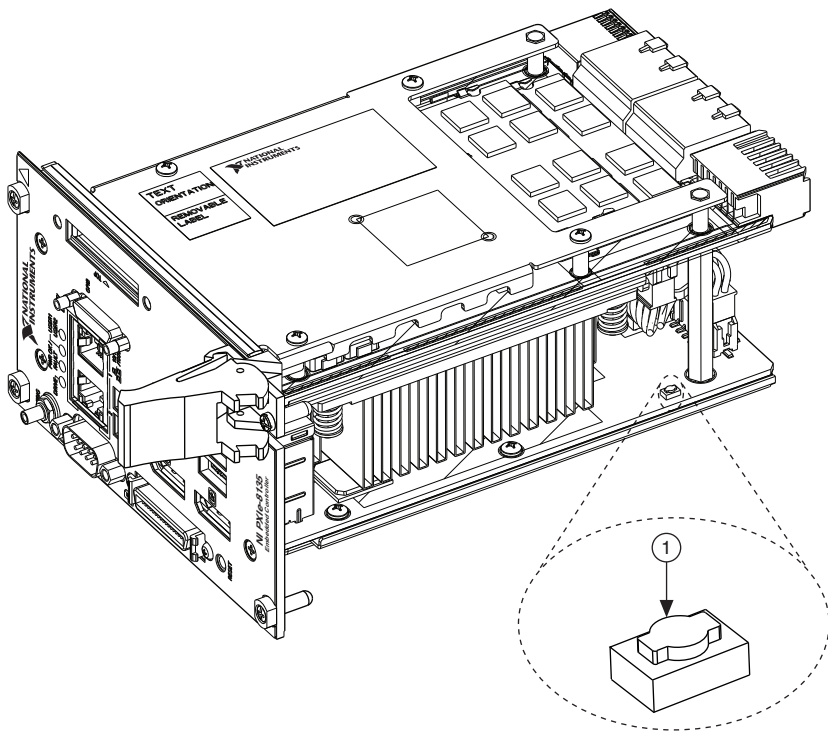
Figure 2-3. Clearing the CMOS Contents
